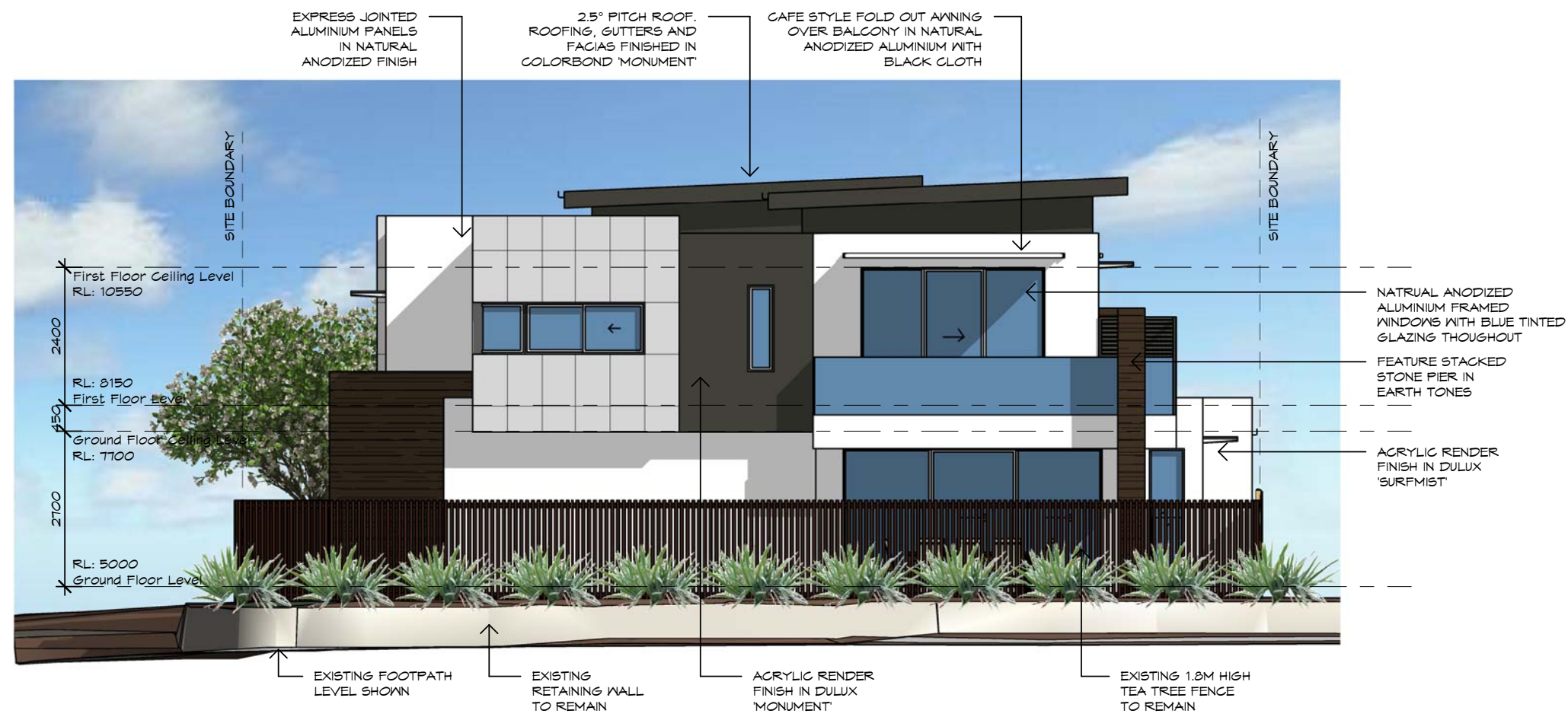
1 East Elevation Page 03 1 : 100
